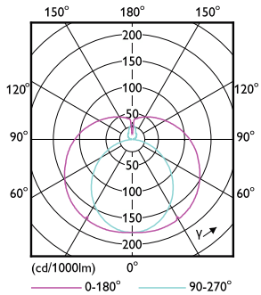
Light Distribution Diagram - MAS LEDtube VLE 1200mm 13.1W/15.5W 865T8
