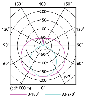
Light Distribution Diagram - MAS LEDtube VLE 1500mm 19.3W/23W 865 T8
