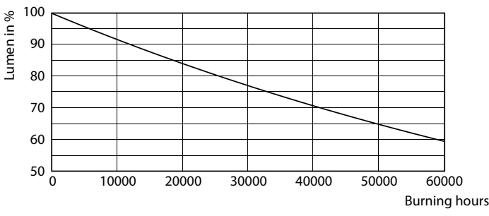
Lumen Maintenance Diagram - MAS LEDspotLV D 7.5-50W 930 MR16 24D
