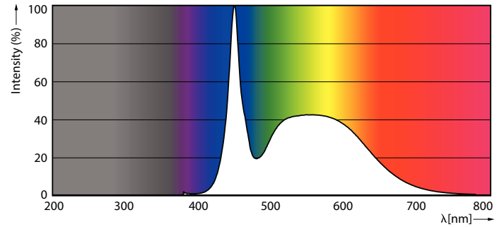
Spectral Power Distribution Colour - LEDtube Connected IA 1500mm 23.1W865 T8
