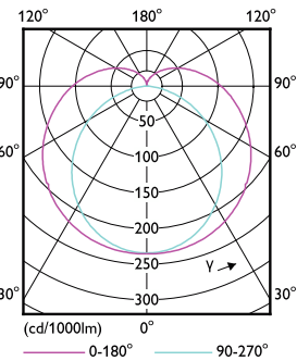
Light Distribution Diagram - MAS LEDtube HF 1200mm UO 16W865 T8
