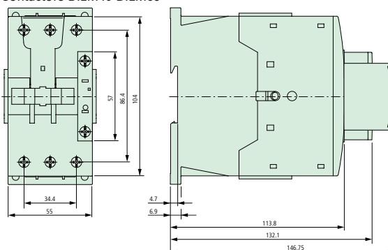
Contactors DILM40-DILM65
