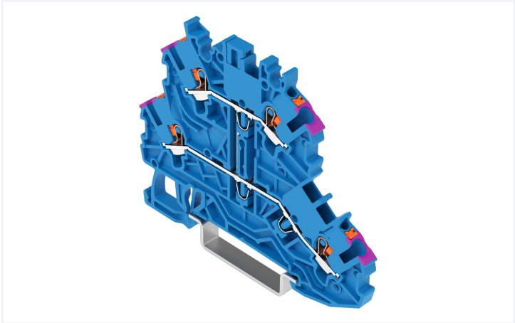
Double-deck terminal block, 2200 Series, blue
