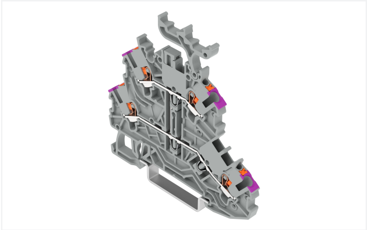
Double-deck terminal block, 2200 Series, gray
