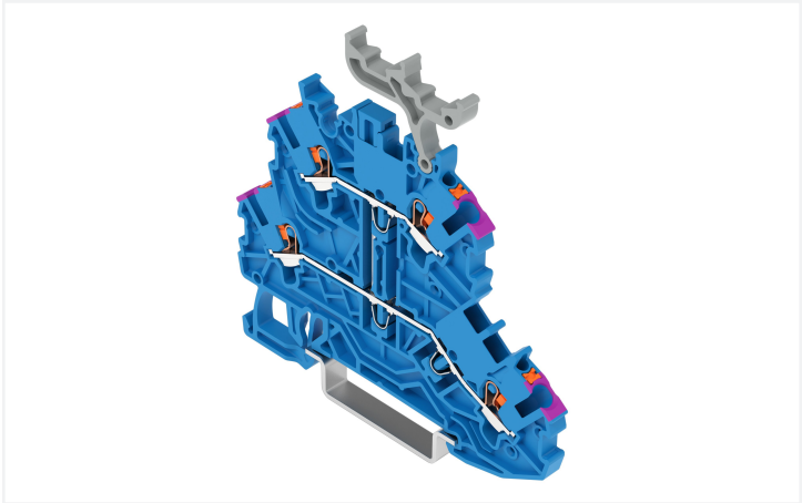
Double-deck terminal block, 2200 Series, push-button
