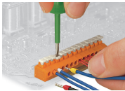
Insert/remove fine-stranded conductors with ferrules via push-button.
