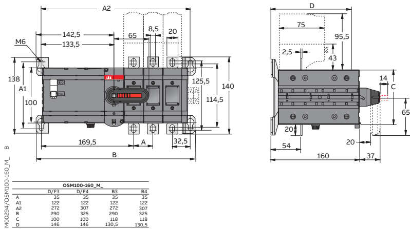
Figure 4.4 OSM100-160_M_
