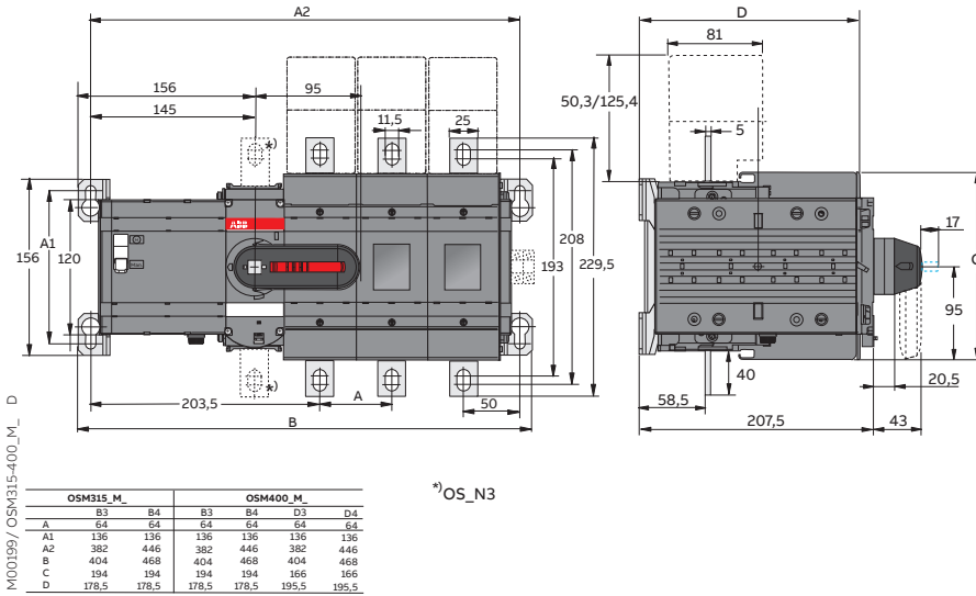
Figure 4.7 OSM315-400_M_
