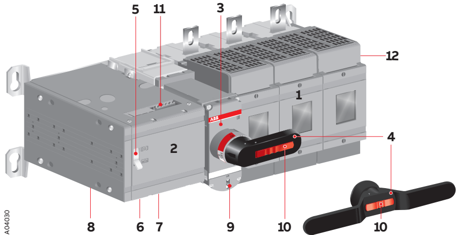
Figure 2.1 Motorized switch fuse (type OSM)
