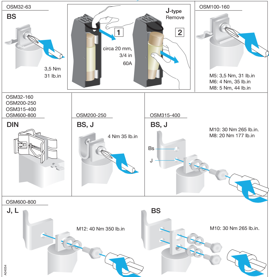
Figure 8.1 Mounting of the different type of fuse links for OSM32-800
