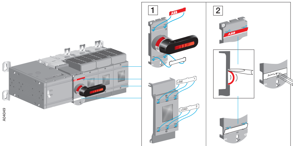
Figure 4.11 Labelling of the motorized switch fuses
