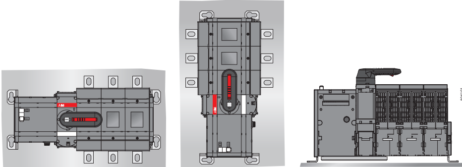
Figure 4.10 Mounting positions
