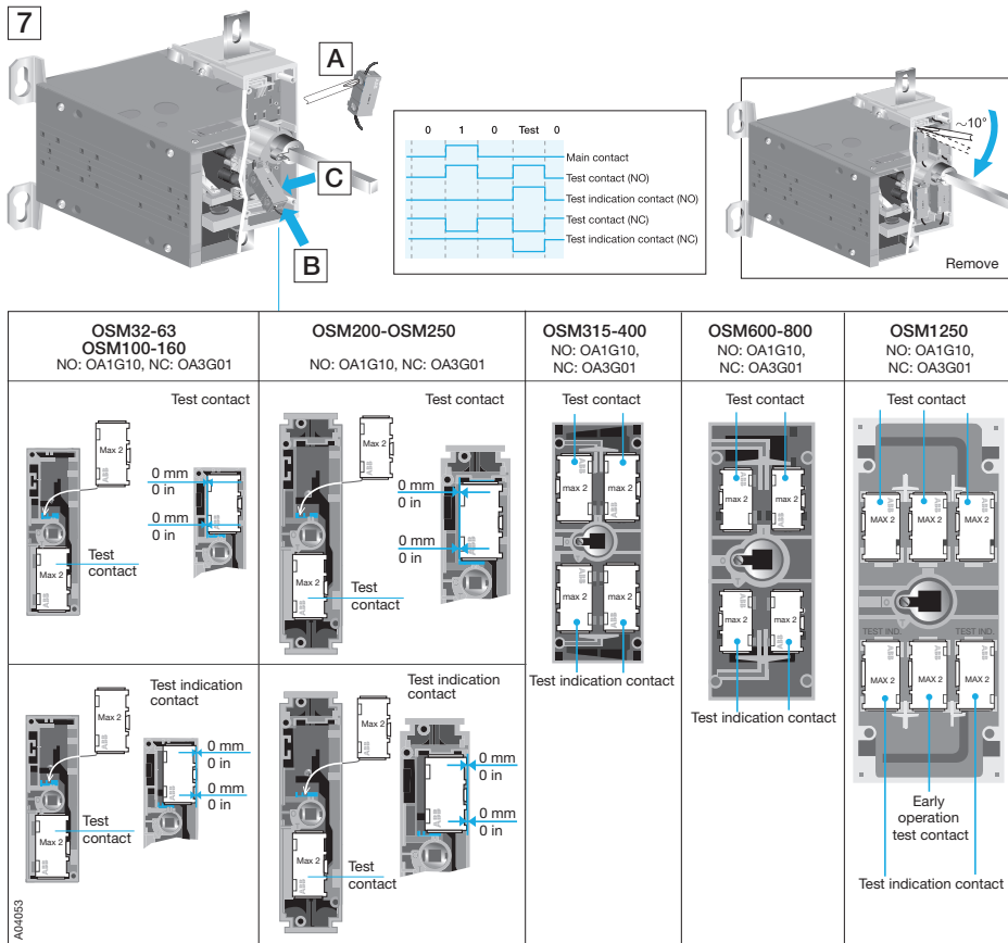
Figure 8.9 Mounting of the Test auxiliary contacts, type OA_ on the switch mechanism
