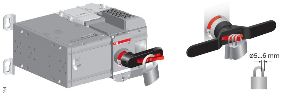
Figure 3.4 Locking the manual operation
