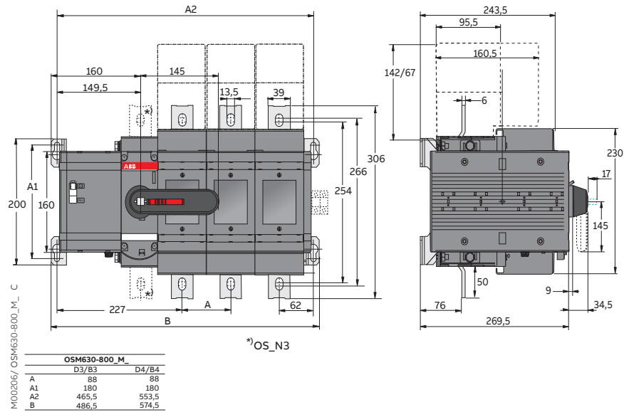
Figure 4.8 OSM630-800_M_
