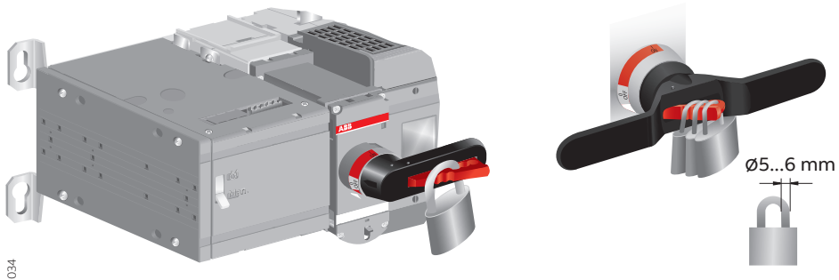
Figure 6.8 Locking the manual operation
