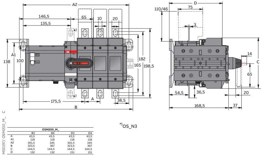
Figure 4.5 OSM200_M_
