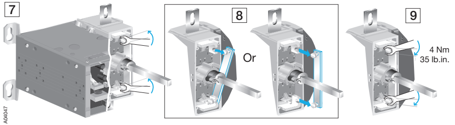
Figure 8.12 Mounting of the detachable neutral links
