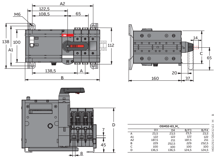
Figure 4.3 OSM32-63_M_
