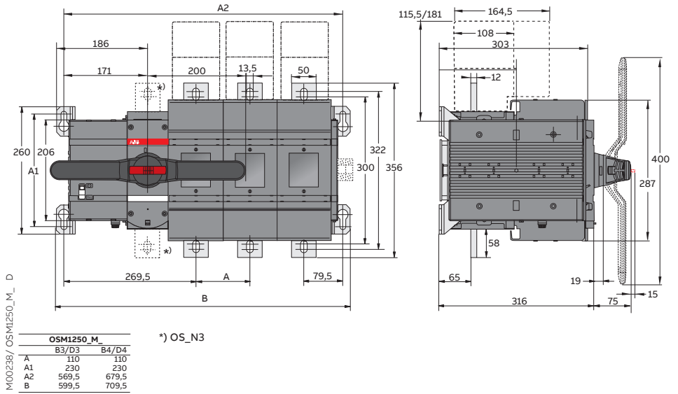
Figure 4.9 OSM1250_M_
