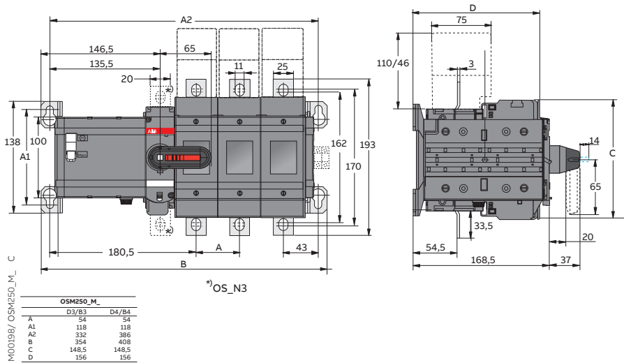
Figure 4.6 OSM250_M_
