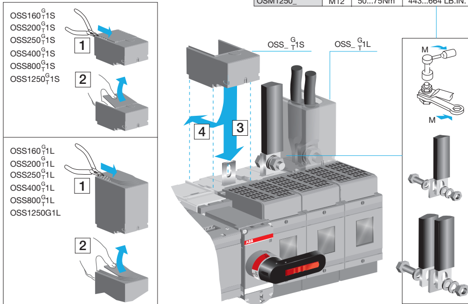
Figure 8.5 Mounting of the terminal shrouds (type OSS_) to the motorized switch fuses
