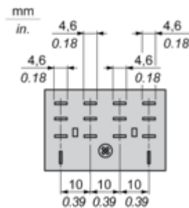
Pin Side View
