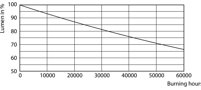
Lumen Maintenance Diagram - MAS LEDBulbND7.3-100W E27 827 A60 CL GUE
