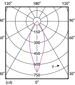
Light Distribution Diagram - MAS LEDspot UE 2.1-50W GU10 ND 827 EELA
