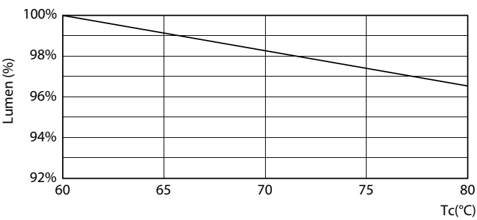
Lumen Maintenance Diagram - MAS LEDtube 600mm HO 10.5W 865 T5
