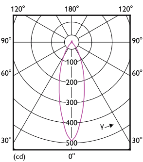
Light Distribution Diagram - MAS LED spot VLE D 2.8-35W GU10 927 36D
