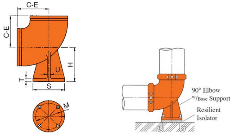
Model 7110-B 90° Elbow, Regular Radius with Base Support
