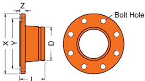
Model 7170 Flange Adapter PN 25
