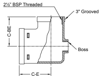
Model 7114 Hydrant Elbow
