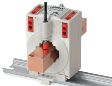
Installation on copper current bar
