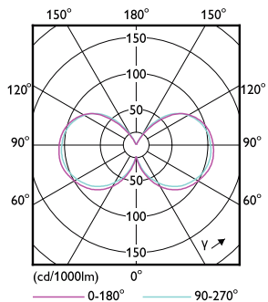
Light Distribution Diagram - MAS VLE LEDBulbD7.2-50W E27 A60 827 CM G
