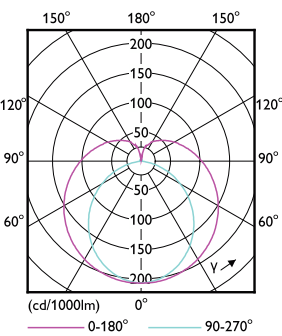
Light Distribution Diagram - MAS LEDtube 600mm HE 7W 830 T5 EU
