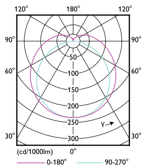
Light Distribution Diagram - LEDtube Connected IA 1500mm 23.1W865 T8
