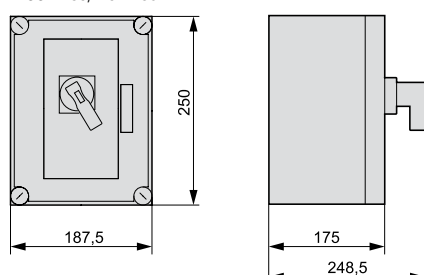
MCCB1-63/I23E-150
