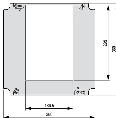
GA-44-S60-XNH1
