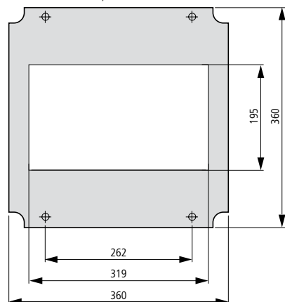
GA-44-S60-XNH00/D02
