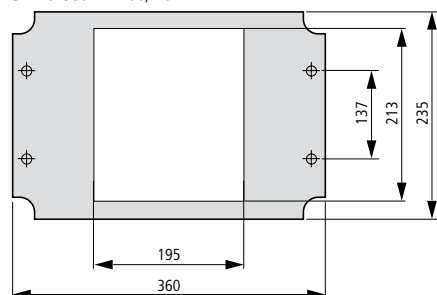
GA-43-S60-XNH00/D02
