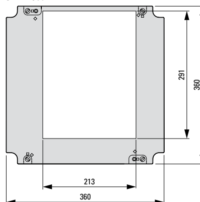
GA-44-S60-XNH2
