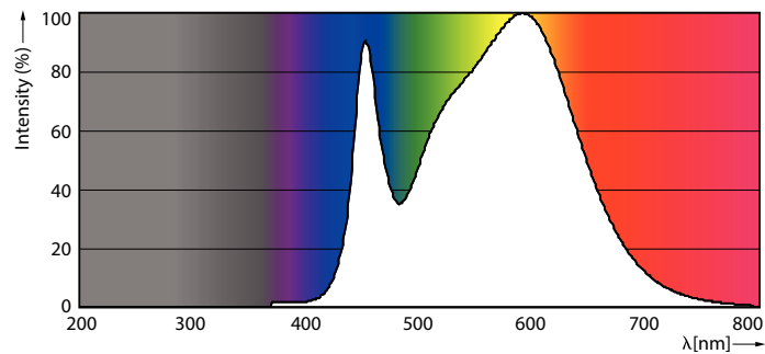
Spectral Power Distribution Colour - CorePro LEDtube UN 1500mm HO 23W840 T8
