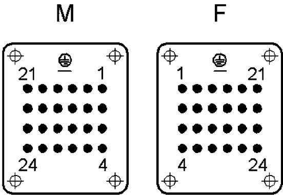
Pin diagram, cable connection side
