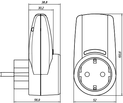
F-Type, Side earthings
