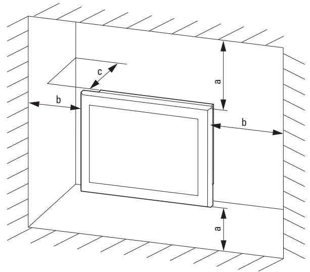
Fig. 15: Mounting distance
