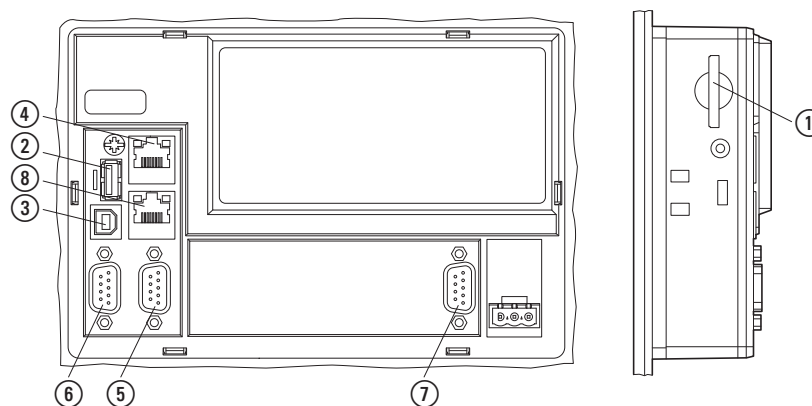
Fig. 25: Basic interfaces on all HMI-PLC units
