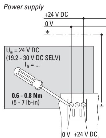
Fig. 23: Connecting the screw terminals on the Plug connector MSTB 2.5/3-ST-5.08
