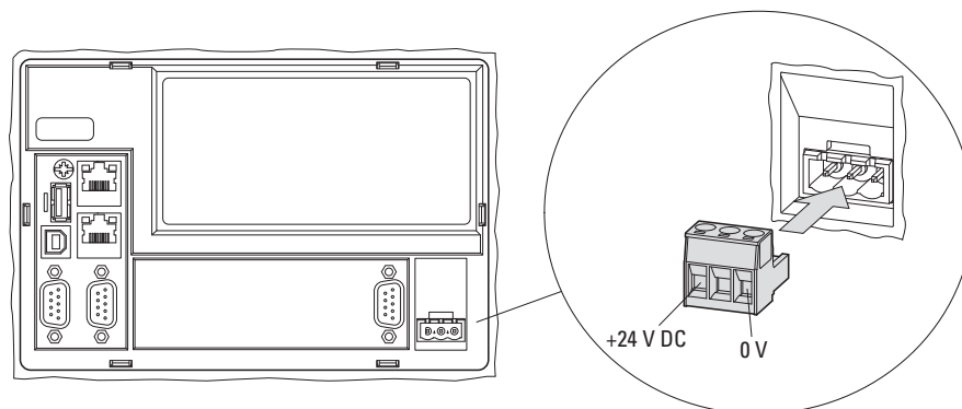
Fig. 24: Power supplied through Plug connector MSTB 2.5/3-ST-5.08
