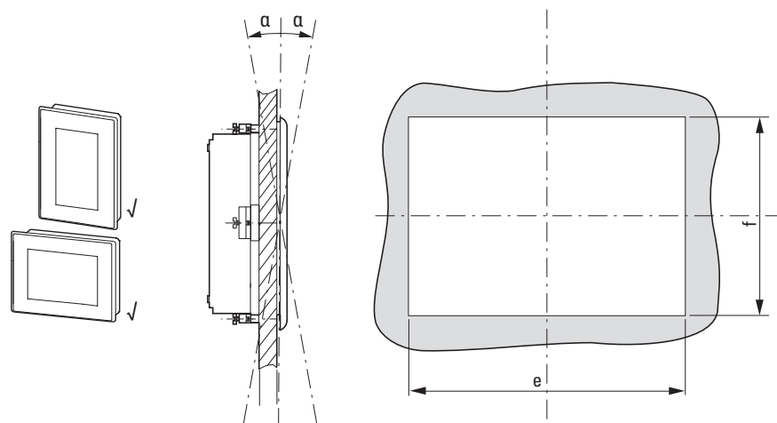
Fig. 16: Mounting position
