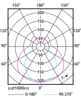
Light Distribution Diagram - CorePro LED PLL EM/Mains 16.5W 840 4P
