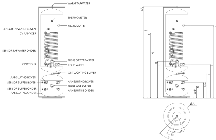
Figuur 5 Tank on Tank boiler
