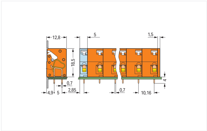
Dimensions in mm Total length = (pole no. – 1) x pin spacing + 5 mm + 1.5 mm
