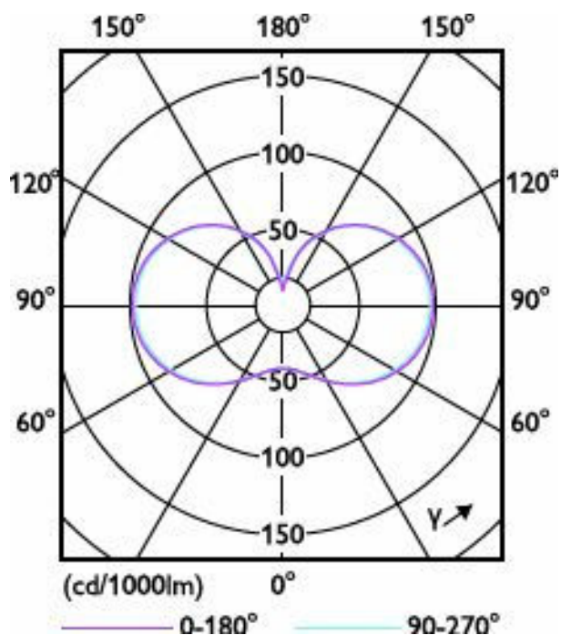
Light Distribution Diagram - TForce Core LED HPL 18W E27 840 FR
