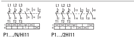
P1.../N/HI11
