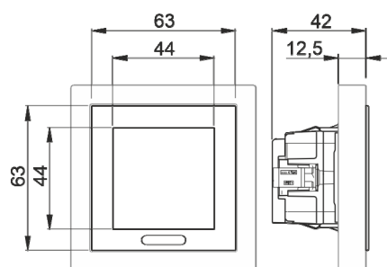
Fig. 6: 2.4" Display 63 SD/U12.63.11-825
