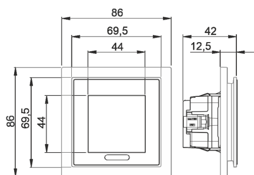
Fig. 8: 2.4" Display 70 SD/U12.70.11-4015
