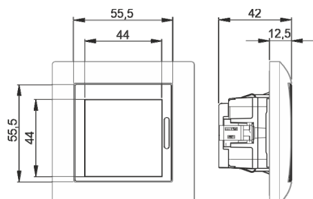
Fig. 5: 2.4" Display 55 SD/U12.55.11-825
