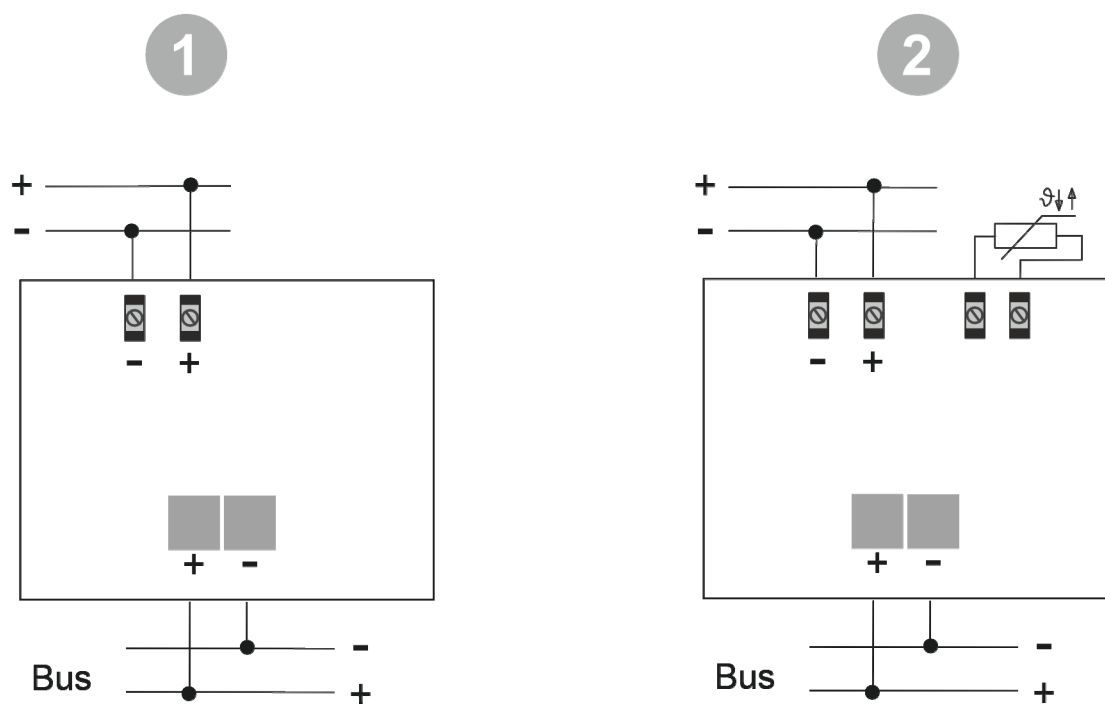
Fig. 9: Electrical connection
