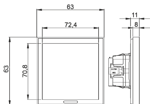
Fig. 7: Busch-RoomTouch® 4" RT/U12.86.11-811
