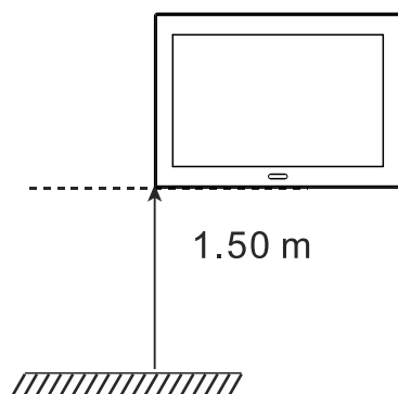
Fig. 12: Mounting height
