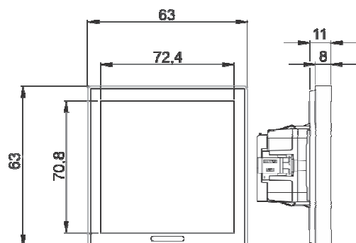
Fig. 7: 4" RoomTouch® RT/U12.86.11-811
