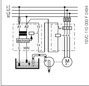
CM-ENE MIN
