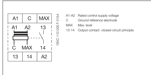
Connection diagram CM-ENN
