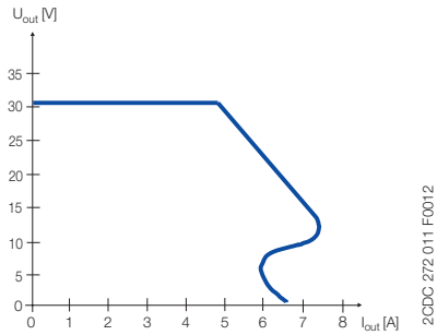
Output behaviour
