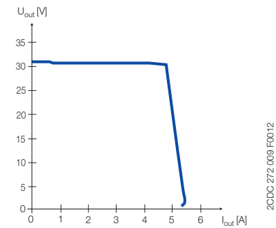
Output behaviour
