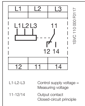
Connection diagram CM-PFE
