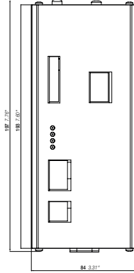
CP-B 24/20.0
