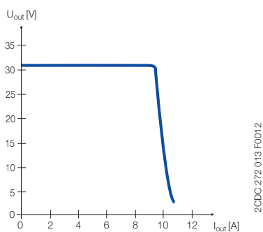
Output behaviour
