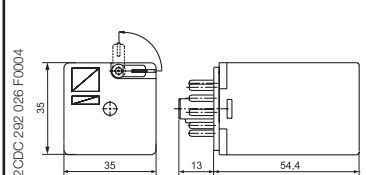
CR-U with 3 c/o contacts
