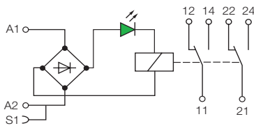
RB/RBR 122 A - 115/230 V AC/DC
