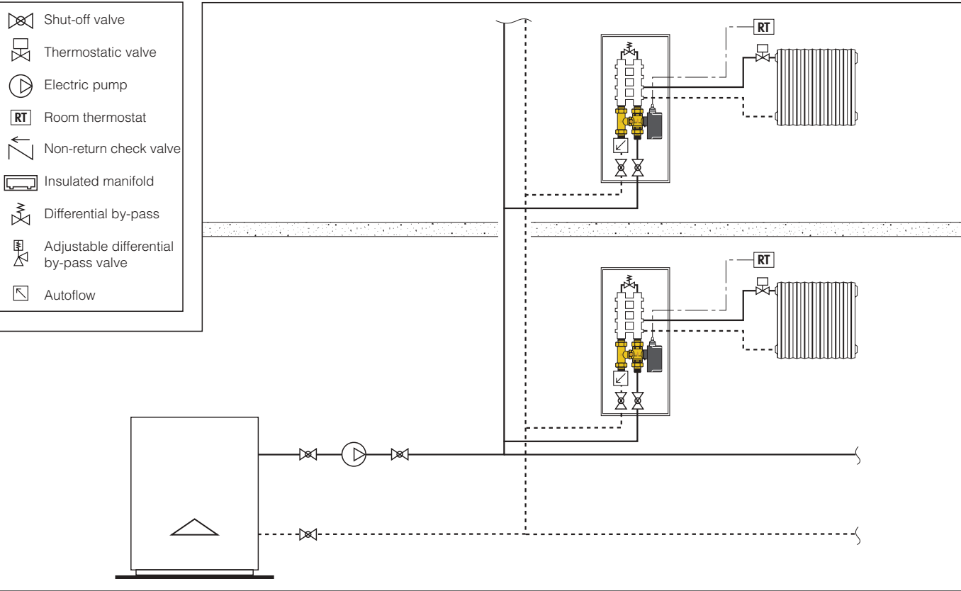
System with 3-way zone valves and Autoflow
