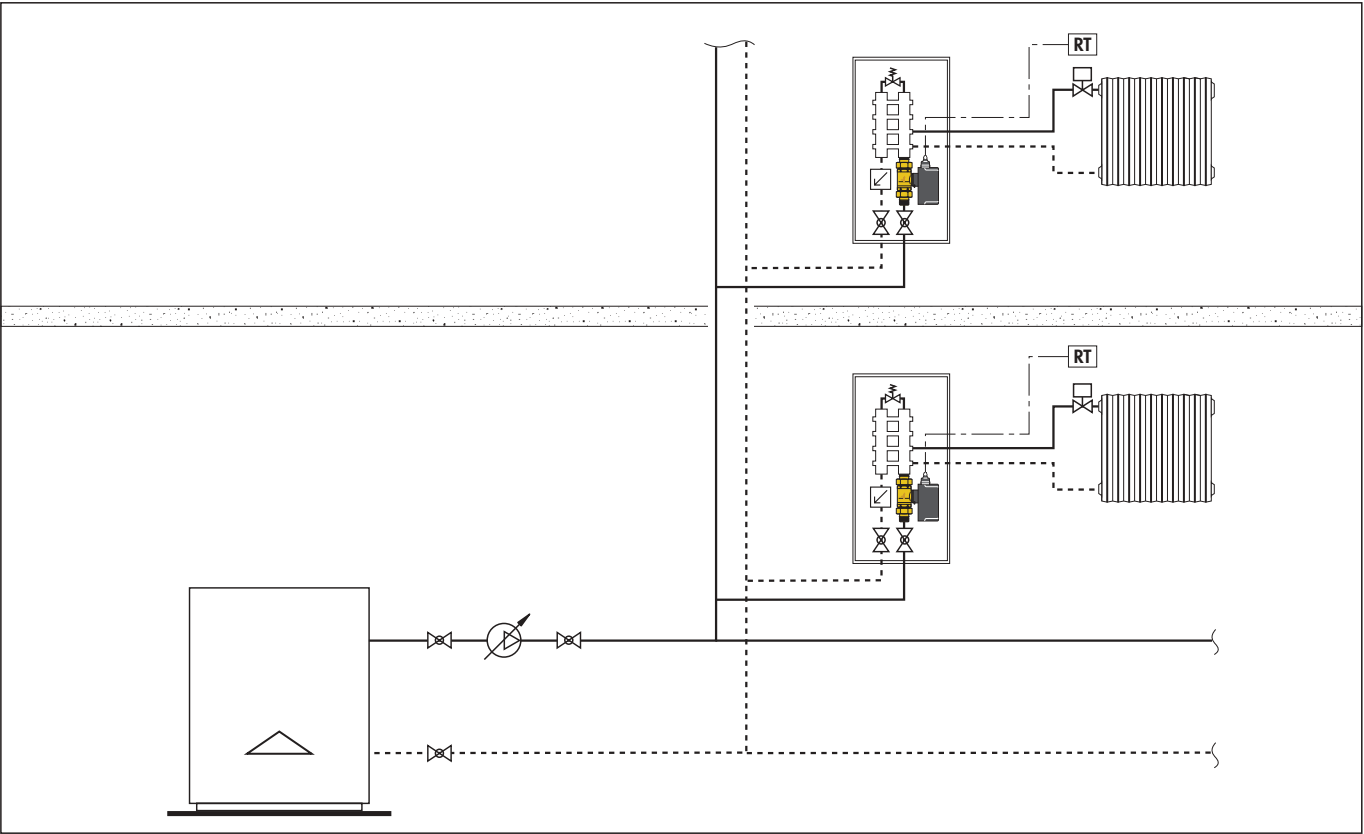
System with 2-way zone valves, variable speed pump and Autoflow
