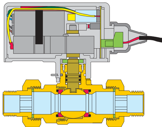
2-way valve, series 6470
