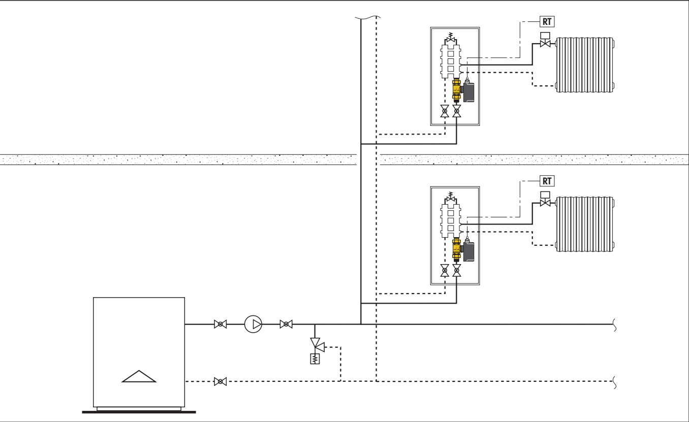
System with 2-way zone valves and adjustable differential by-pass valve
