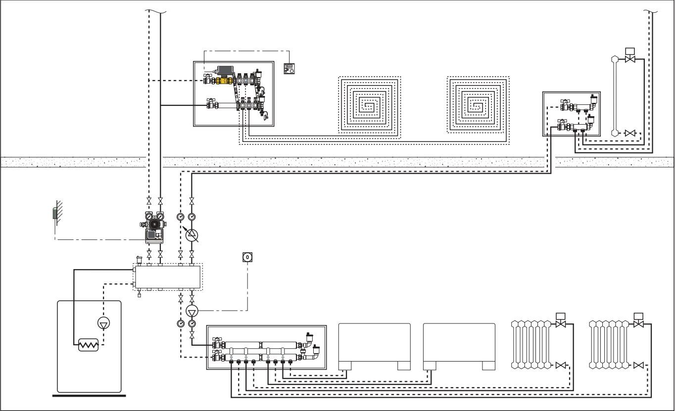
System with 2-way zone valves, temperature regulating unit and Sepcoll
