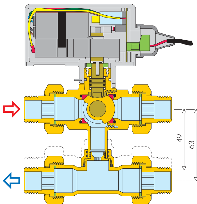
4-way valve, series 6489
