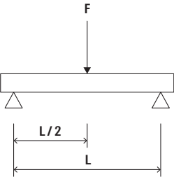
Load case 1
