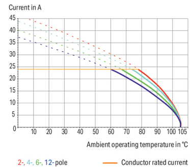
Current-Carrying Capacity Curve
