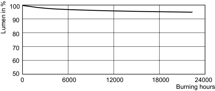
Lumen Maintenance Diagram - SOX 135W BY22d 1SL/12
