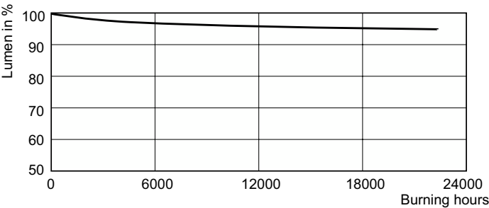
Lumen Maintenance Diagram - SOX 55W BY22d 1SL/12
