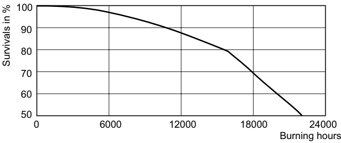
Life Expectancy Diagram - SOX 55W BY22d 1SL/12
