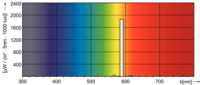
Spectral Power Distribution Colour - SOX 55W BY22d 1SL/12
