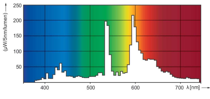
Spectral Power Distribution Colour - CDM-Rm Elite Mini 20W/830 GX10 MR16 25D
