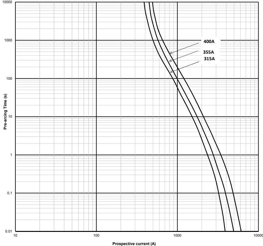
Time-current curve size 3 - 315 A to 400 A
