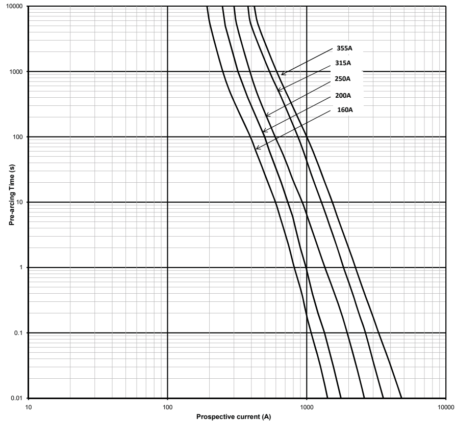
Time-current curve - 1000 V d.c. - 2XL - Bladed and bolted - 160 A to 355 A
