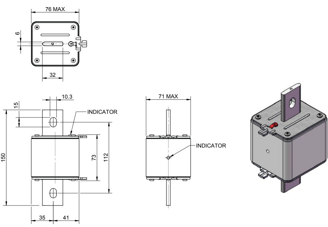
Dimensions (mm) NH3 Blade with bolt holes and lugs
