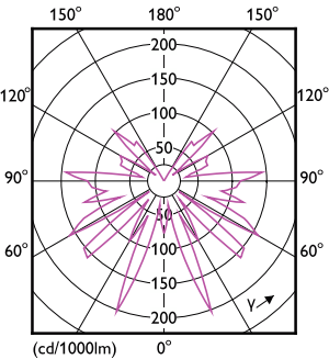
Light Distribution Diagram - MAS VLE LEDLusterD 2.6-15W E14 P45 SP G
