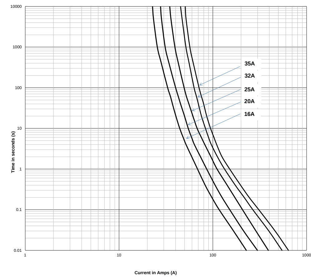
Time-current curves - NH Size 00 16 to 35 Amps
