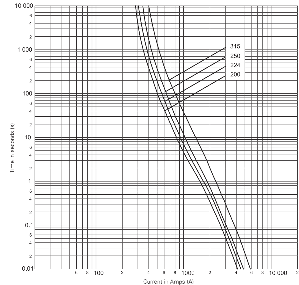
Technical data - NH size 2
