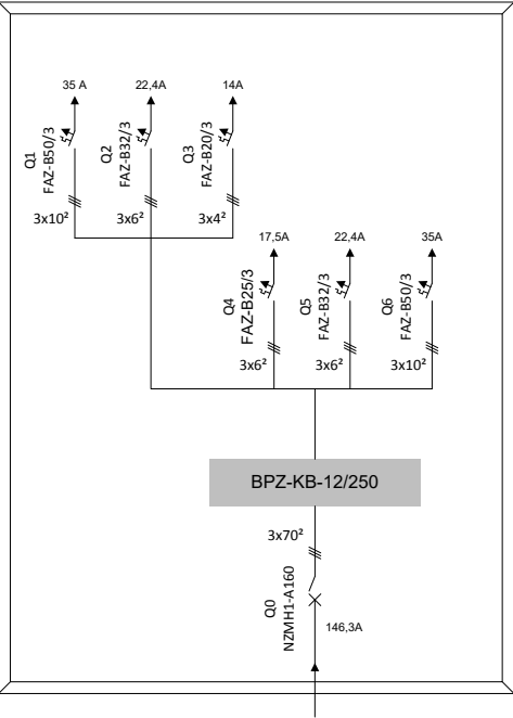
Single-line diagram of the assembly with rated current ≤ 160 A:
