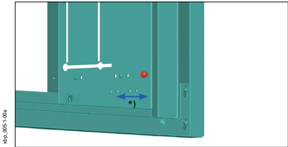
Detail of bottom hitch *) possibility of change of side wall depth
