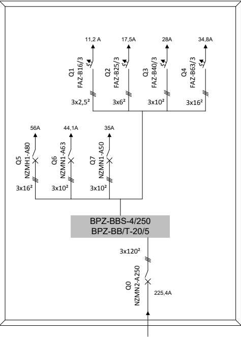
Single-line diagram of the assembly with rated current ≤ 250 A:
