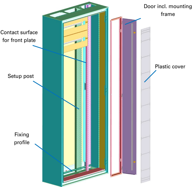
Example of application (floor-standing enclosure IP55 in a width of 800 mm incl. cable area of 200 mm)
