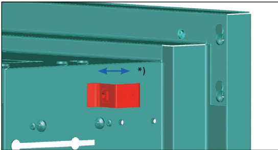
Detail of top hitch
