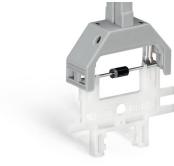
Pressing component into plug contact via operating tool
