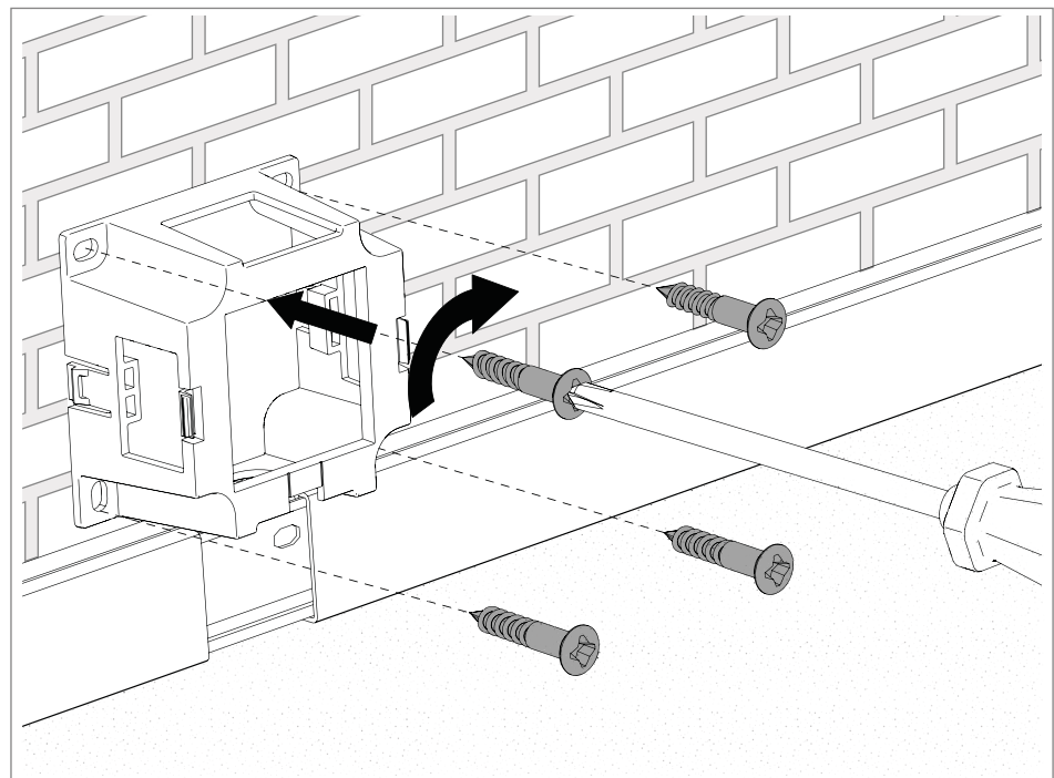
Fig. 29: Mounting the basic body
