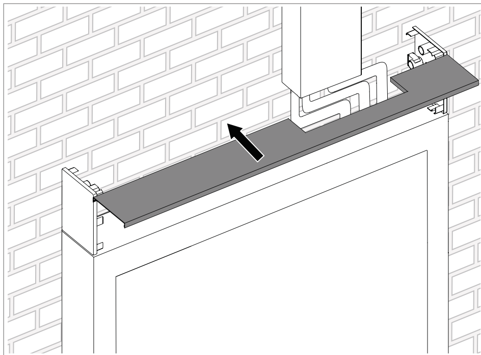
Fig. 48: Installing covers
