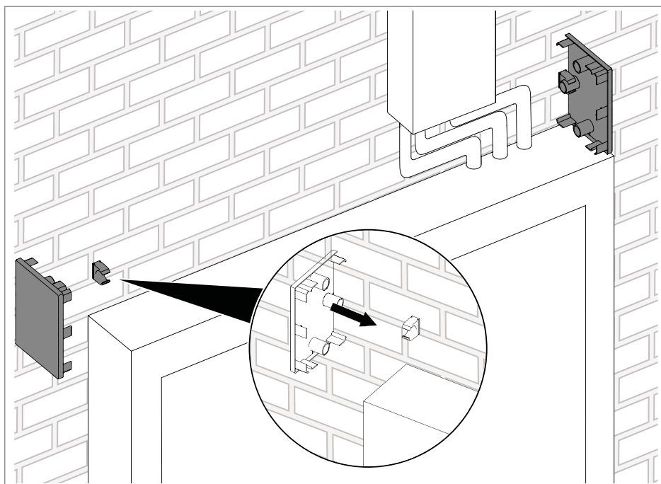
Fig. 46: Mounting end pieces
