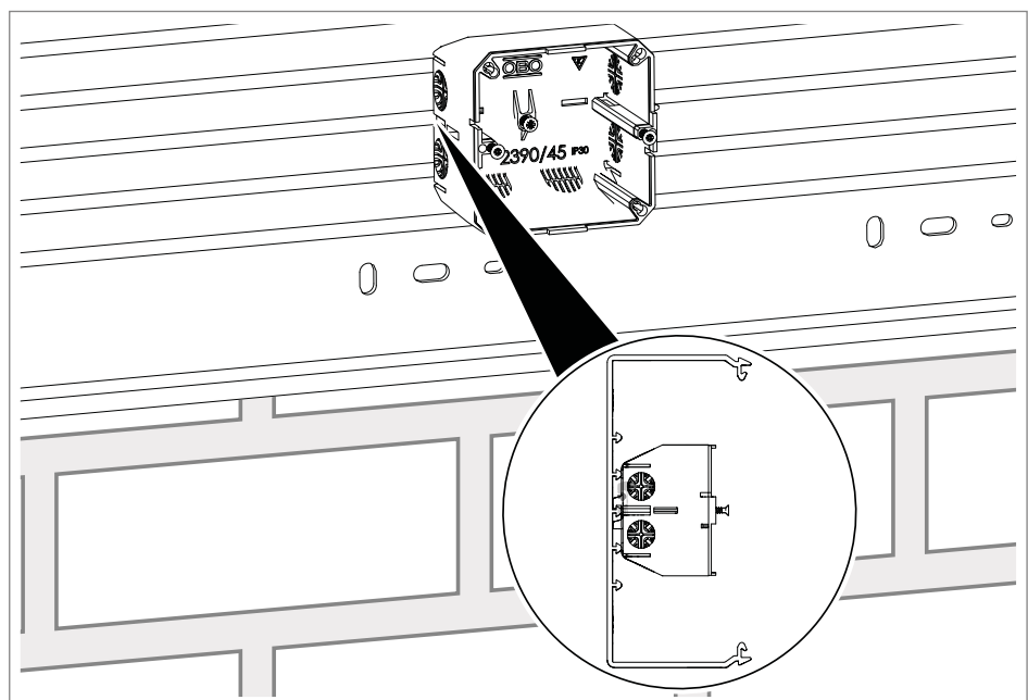
Fig. 16: Mounting the device installation socket for Schuko sockets
