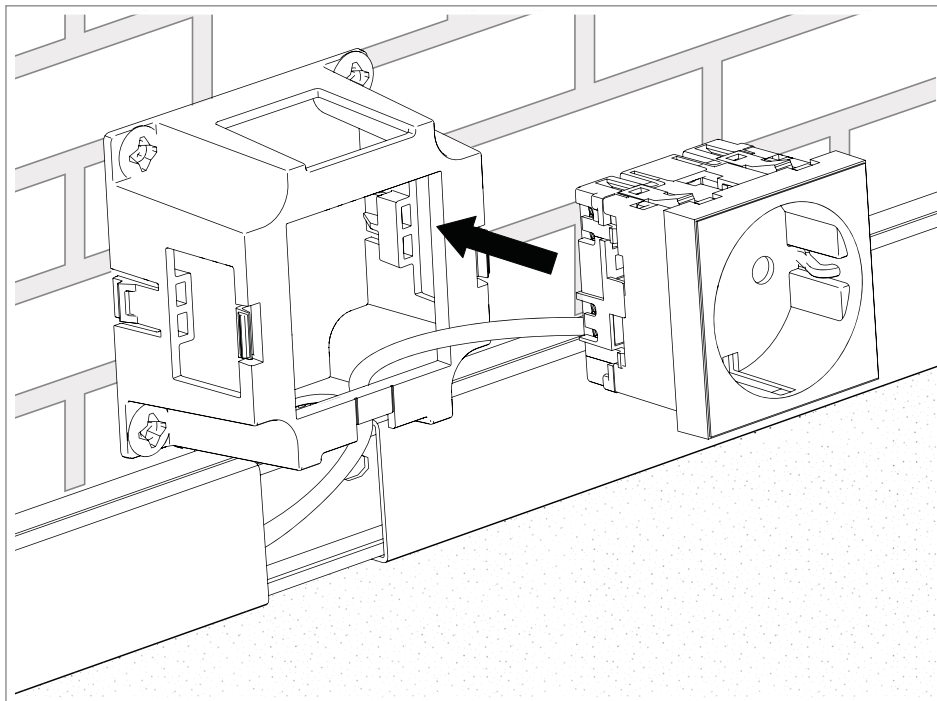
Fig. 30: Installing the socket
