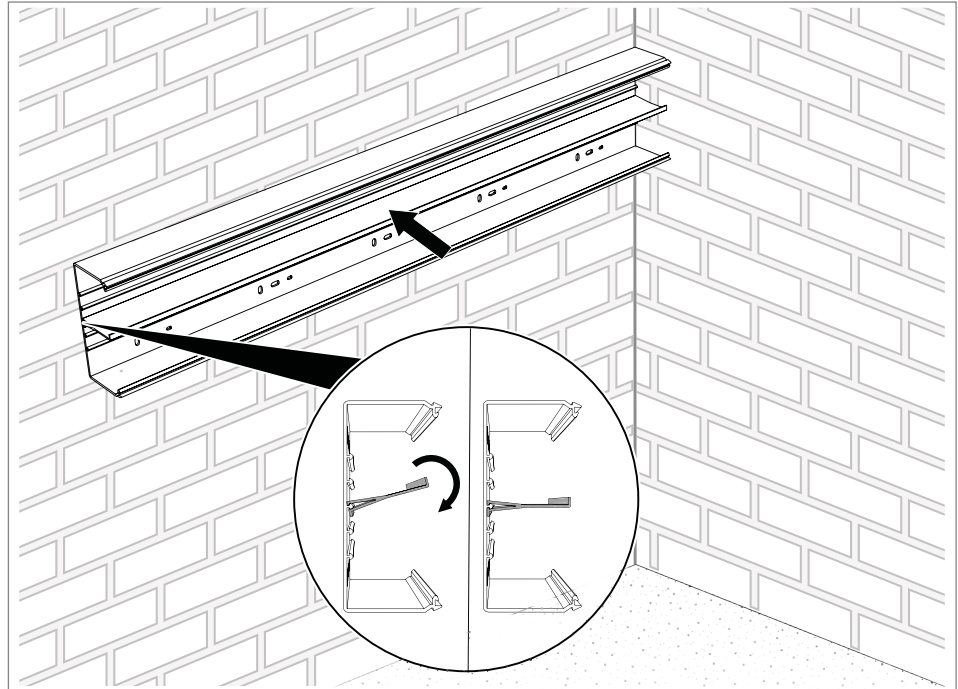
Fig. 12: Mounting the partition
