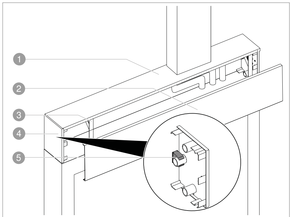
Fig. 44: Universal trunking
