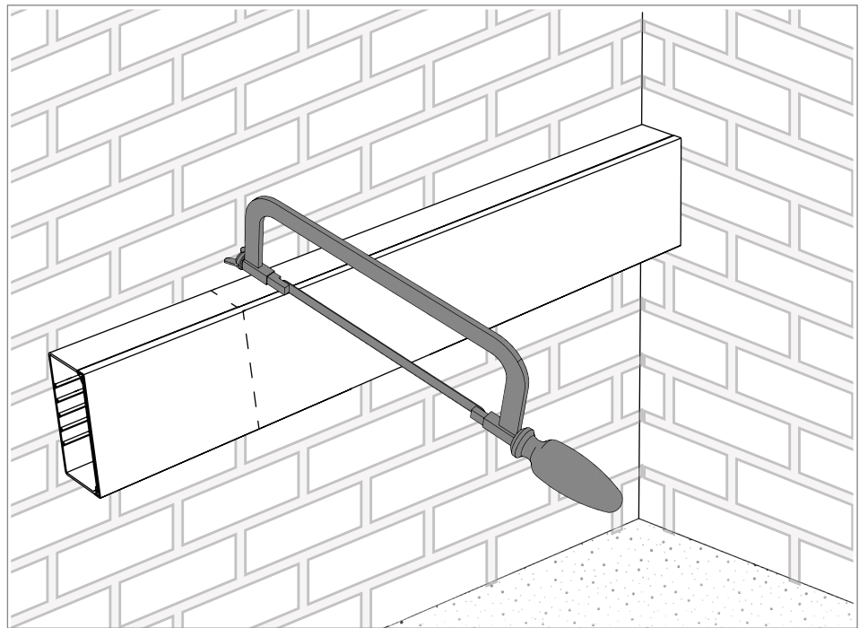
Fig. 7: Adjusting the WDK cable trunking
