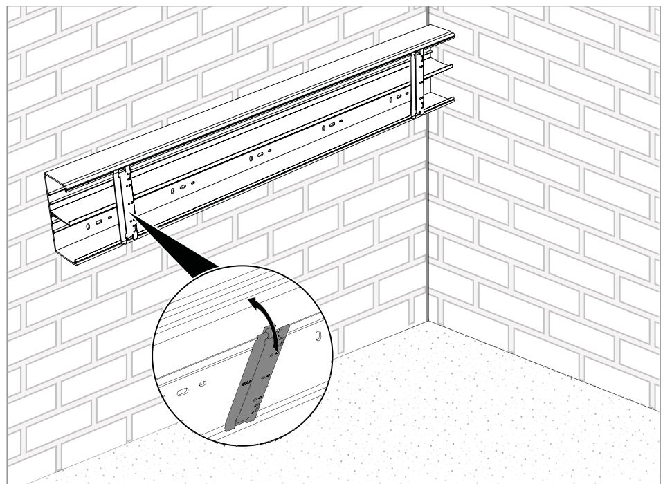
Fig. 13: Mounting cover clips
