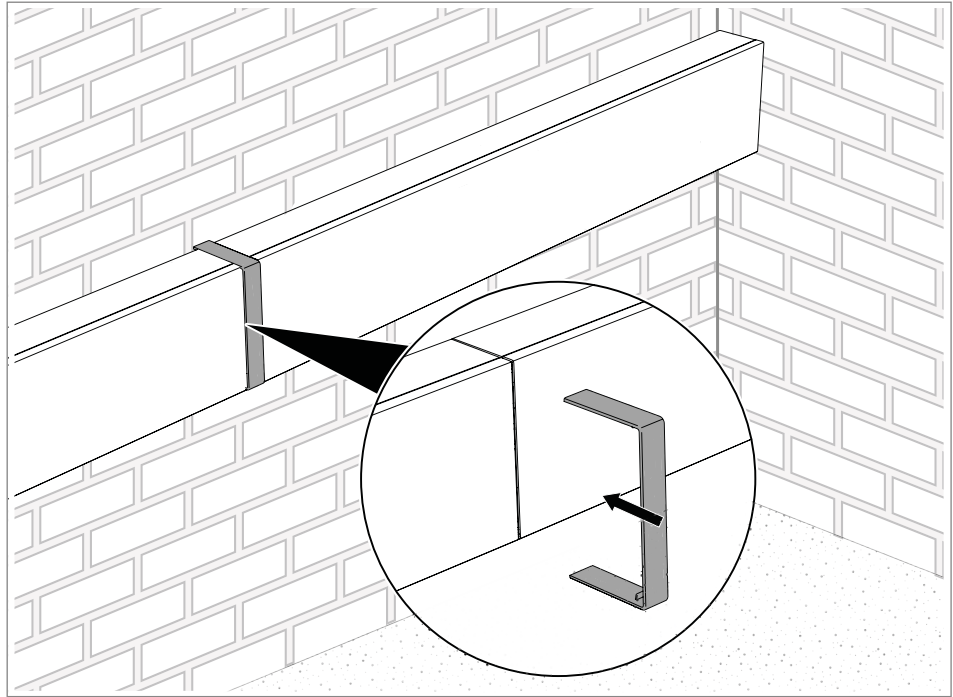
Fig. 43: Mounting the joint cover
