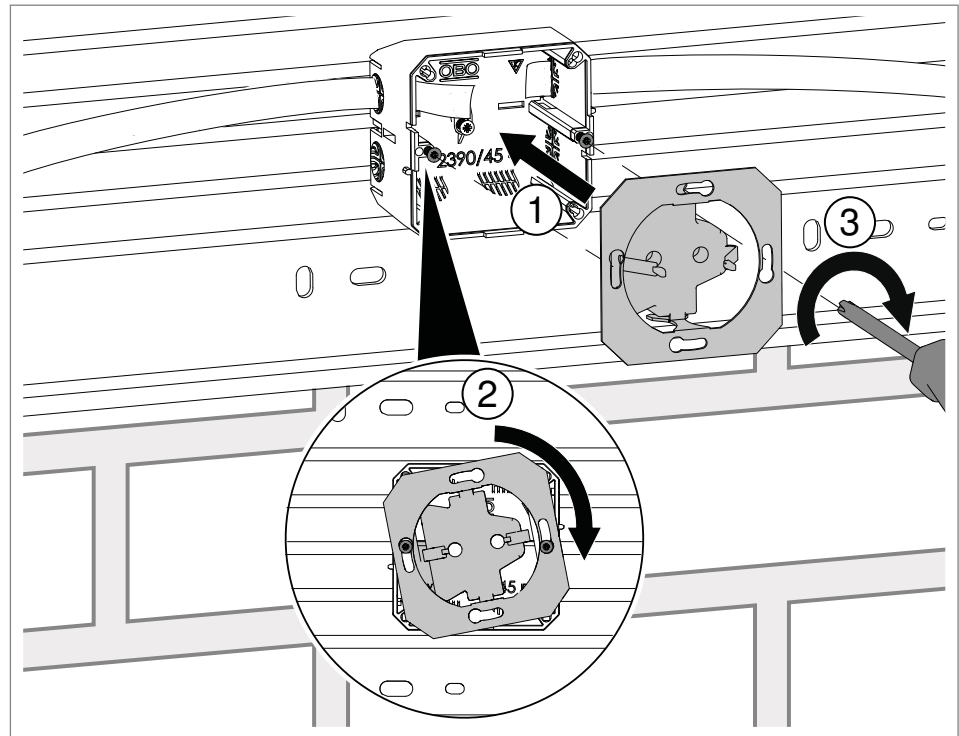
Fig. 19: Connecting the socket
