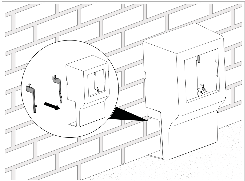
Fig. 27: Inserting the adapter plate
