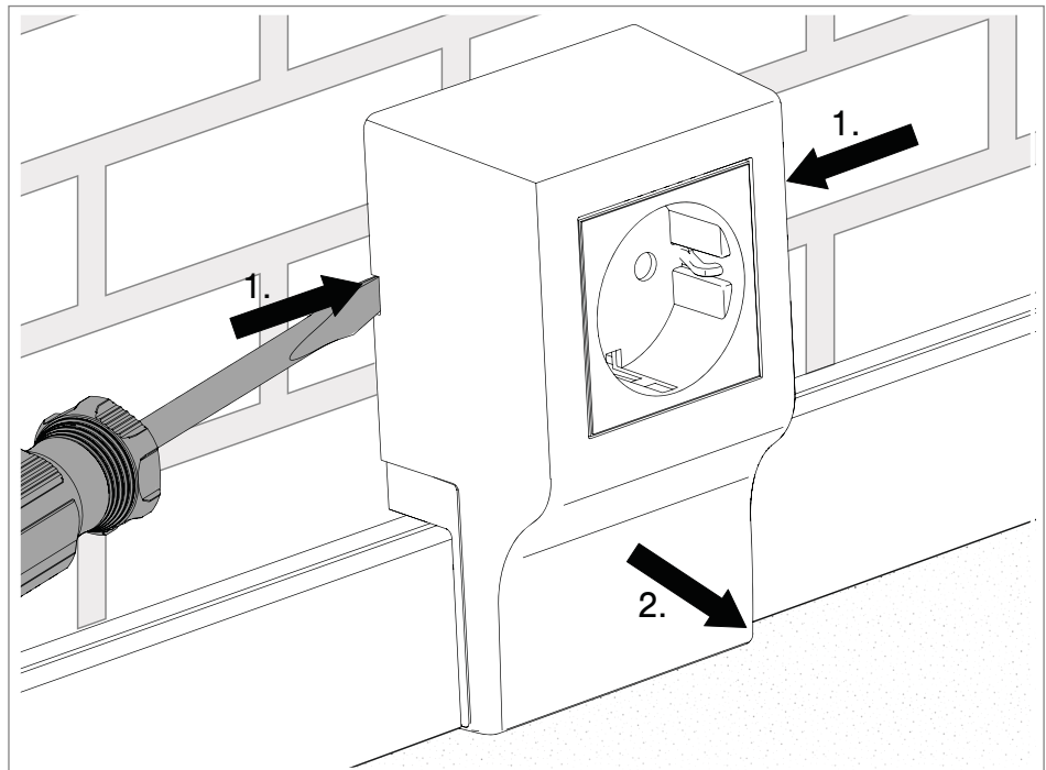
Fig. 32: Dismantling the device support
