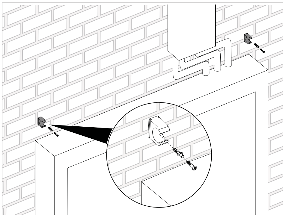
Fig. 45: Mounting fastening clips
