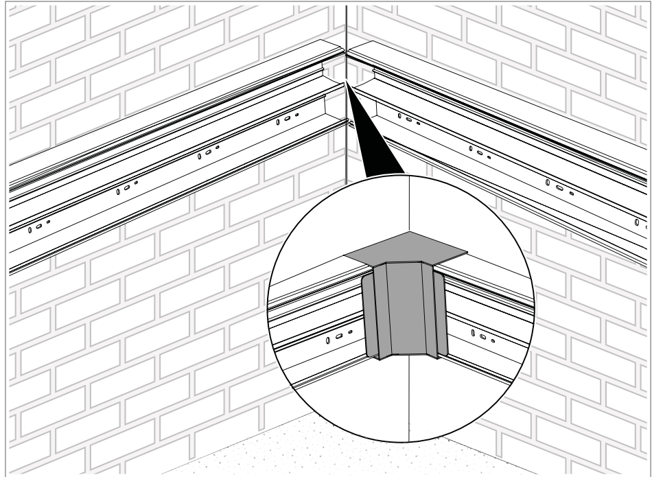
Fig. 33: Mounting the internal corner cover
