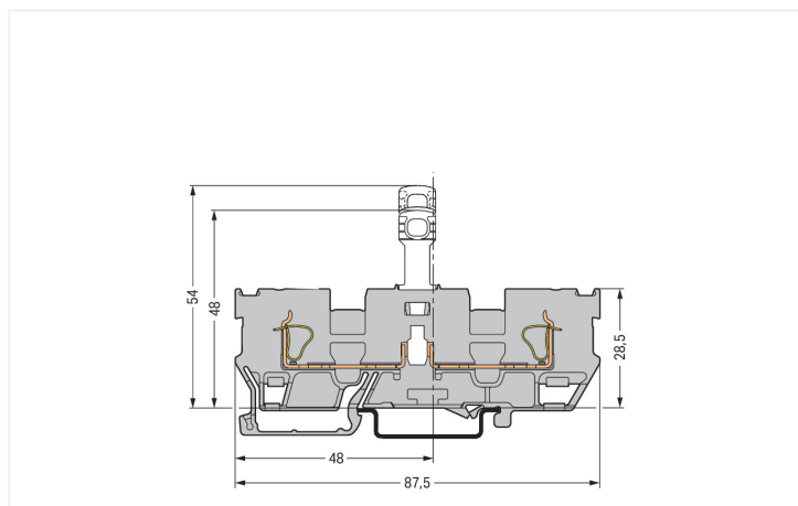
Disconnect carrier terminal block
