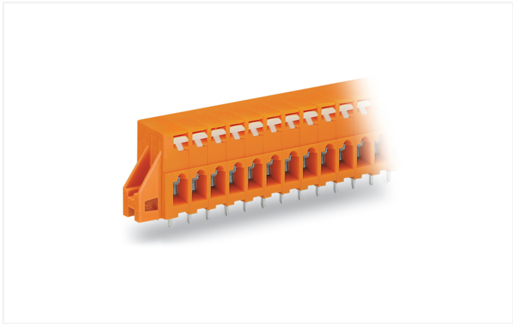
Color: ■ orange Similar to illustration Dimensions in mm L = (pole no. – 1) x pin spacing + 6.5 mm + 1.5 mm L1 = L + 5.8 mm L2 = L1 + 6 mm
