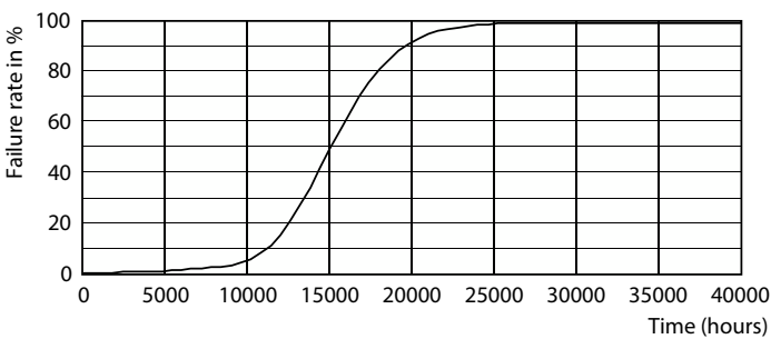
Life Expectancy Diagram - TForce Core HB MV ND 30W E27 830 G3
