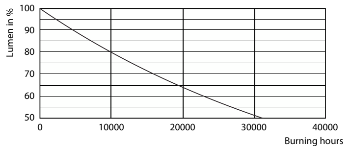
Lumen Maintenance Diagram - CorePro LED linear D 14-120W R7S 118 840
